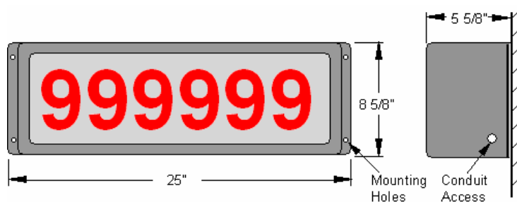
Option 1: Surface Mount Back Panel
